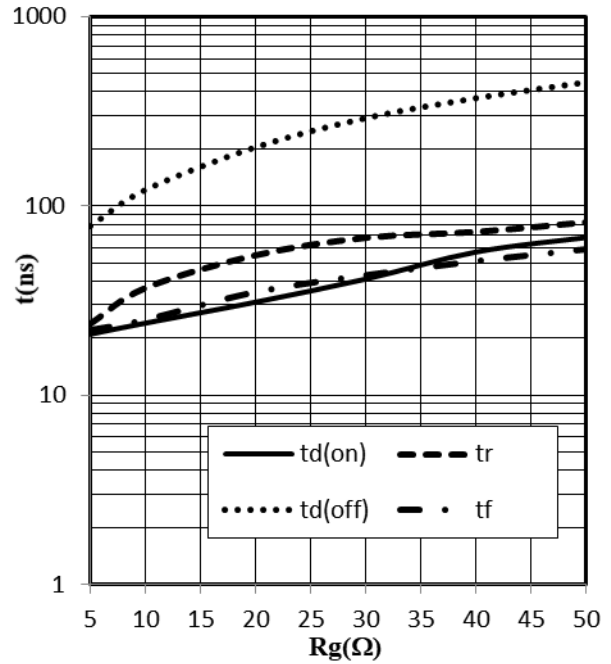
Fig 14. Typical switch time as a function of R_G (inductive load, T_J=25^\circ\text{C} , V_{CE}=400\text{V} , V_{GE}=15\text{V} , I_C=30\text{A} )
