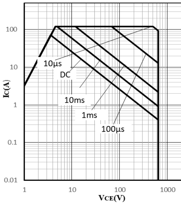
Fig 3. IGBT Forward safe operation area
