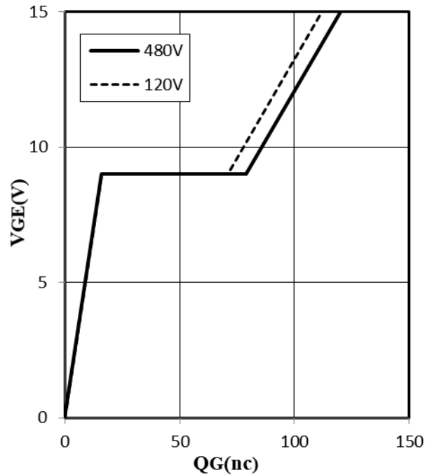
Fig 16. Typical gate charge ( I_C=30\text{A} )
