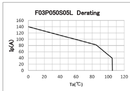
Figure 6: Ip vs Ta for F03P050S05L
