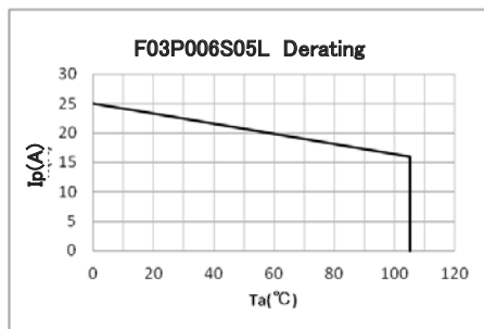
Figure 3: Ip vs Ta for F03P006S05L
