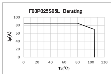
Figure 5: Ip vs Ta for F03P025S05L
