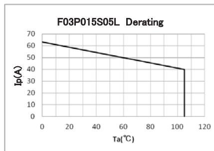
Figure 4: Ip vs Ta for F03P015S05L
