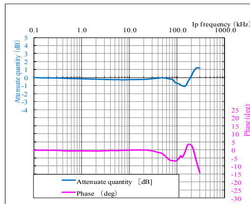
Figure 2: Frequency response curve
